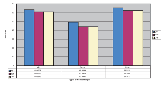
Graph forAverage Blurr and Various Deblurring techniques
