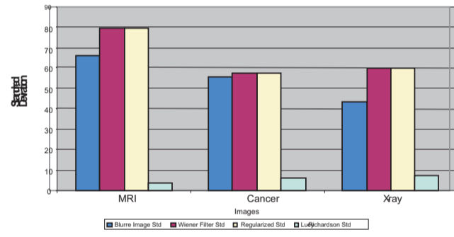
Graph forPrewitt Blurr and Various Deblurring techniques
