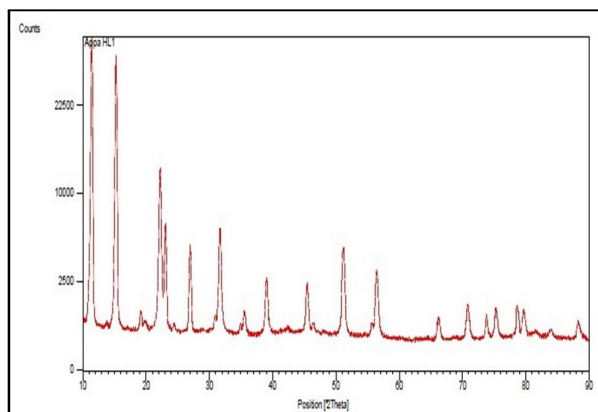
Fig.-2: X-Ray Diffraction Pattern of NiHL1 Metal Complex
