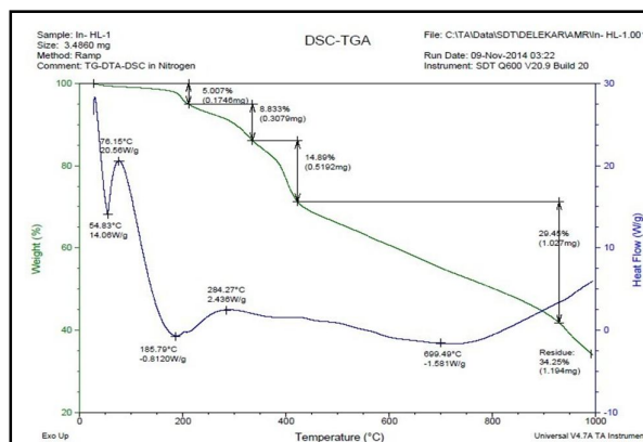
Fig.-1: Thermal Analysis of Nickel Complex
