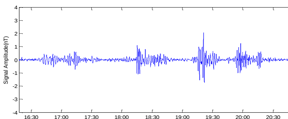
Figure 1: Filtered time series of selected data of 28th Jan.-2005(Hanle) in UT
