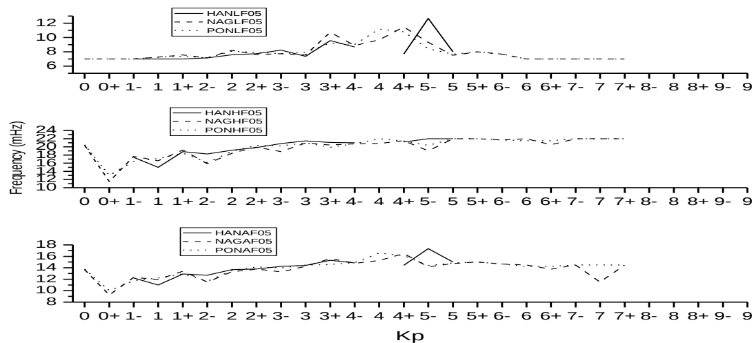
Figure: 4 Seasonal alterations in frequency of Pc4 occurrence at all three stations Hanle (HAN), Nagpur (NAG) and Pondicherry (POND) in summer season 2005
