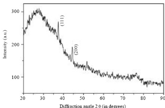
Fig. : X-Ray diffraction range of blended silver nanoparticles
